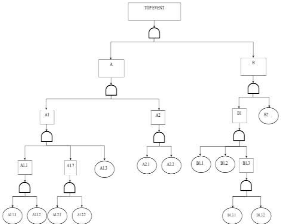
Lampiran 3 Diagram Fault Tree Analysis
