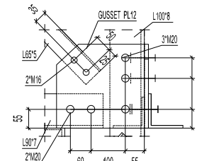
DETAIL "2"
