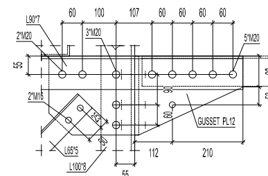
DETAIL "1"
