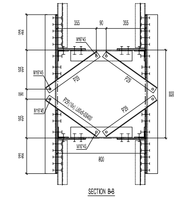
SECTION B-8
