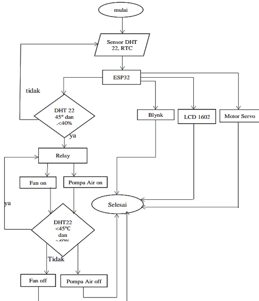
Gambar 2. Flowchart Software
