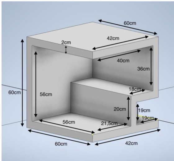
Lampiran 1. Desain cold storage 3D.
