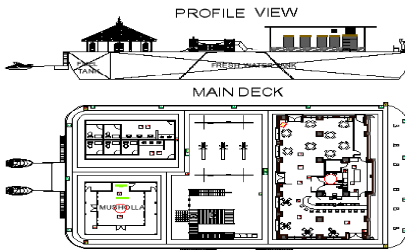
Figure 3. General Arrangement
