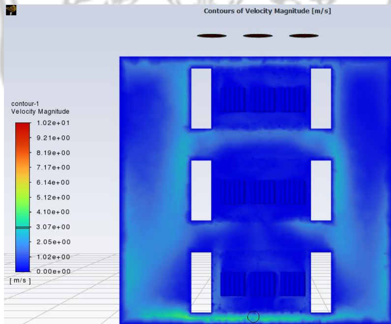
Lampiran 5. Kontur velocity magnitude potongan sumbu ZX oven 4 exhaust layer 3.
