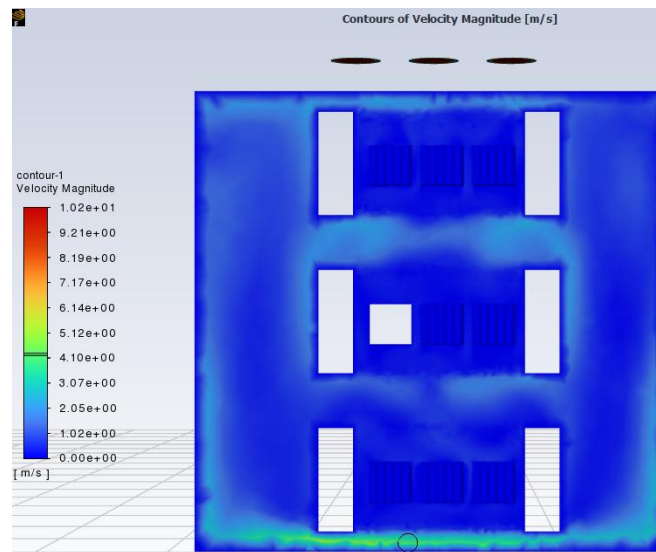
Lampiran 7. Streamline vector velocity potongan sumbu ZX oven 4 exhaust.
