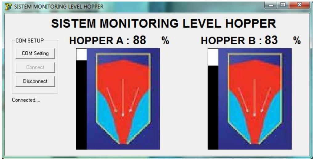
Gambar 4.3 Tampilan Monitoring Program Borland Dhelpi di PC
