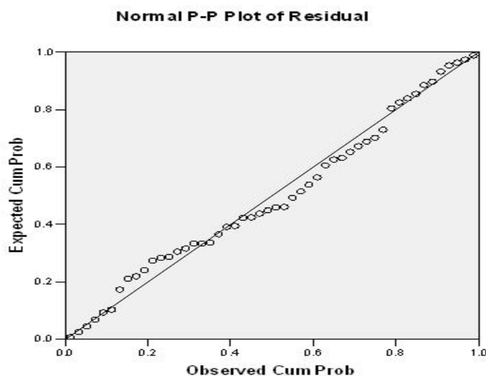
Gambar 3.1. Grafik normal probability plot
