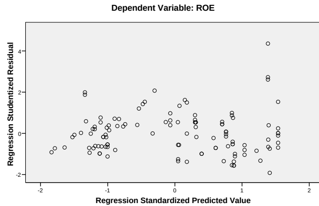
Scatterplot
