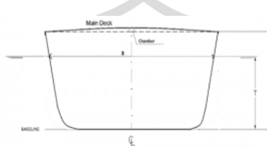
Picture5Ship Width
